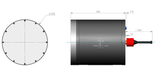
Integrated Head (standard configuration)
