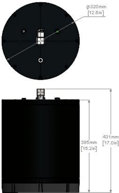
Integrated Head Option
