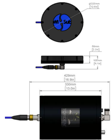
Remote Head (optional configuration)
